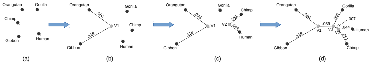
Figure 3. Illustration of iteratively constructing a phylogenetic tree using the NJ algorithm. Distances between mitochondrial DNA sequences of five primate species 37 are used in this example. The NJ algorithm starts from where all five species are separate, as shown in (a). It then selects two nodes based on current pairwise distances to connect to a newly created parent node with calculated edge lengths, as shown in (b). The parent node now represents itself and its two children to calculate distance with every other node in this corpus. This process iterates until there are only three nodes left (V1, V2, and Gorilla ), as shown in (c). The final step is to create a last node to connect the remaining three nodes together to finish the tree construction. V3 is the last created node in (d). The resulting tree has the nodes representing five primate species as leaves, while newly created parent nodes (V1, V2, and V3) possess internal positions.
